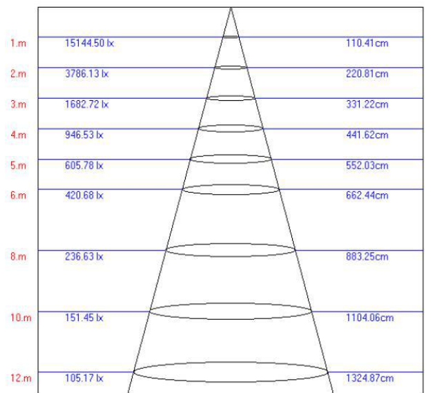
Lux-Distance Curve
